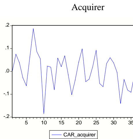
Figure 1. Cross-sectional average of the CAR_{iT+k} evaluated for a 7 days symmetric event windows
