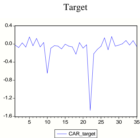
Figure 1. Cross-sectional average of the CAR_{iT+k} evaluated for a 7 days symmetric event windows
